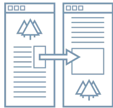
Content migration
